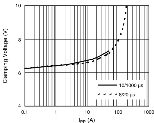
Fig. 4 - Clamping Voltage vs. Peak Pulse Current ( T_J initial = 25\text{ }^{\circ}\text{C} )
